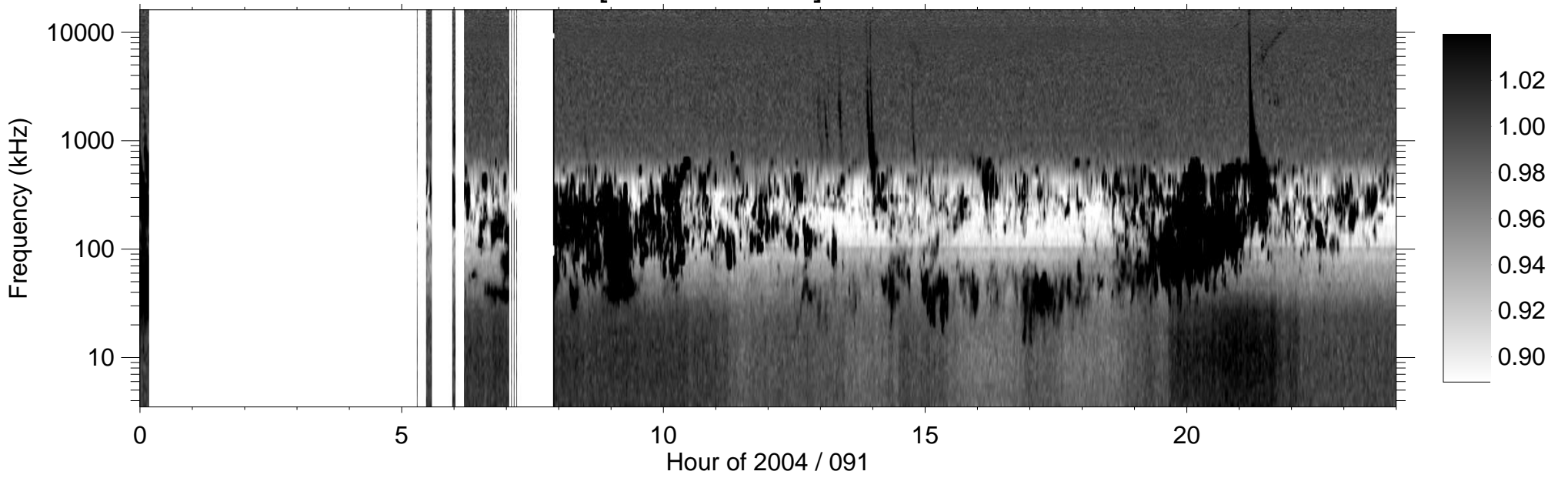
RPWS [ABCH1H2/Ex] (-B) 2004/03/31
