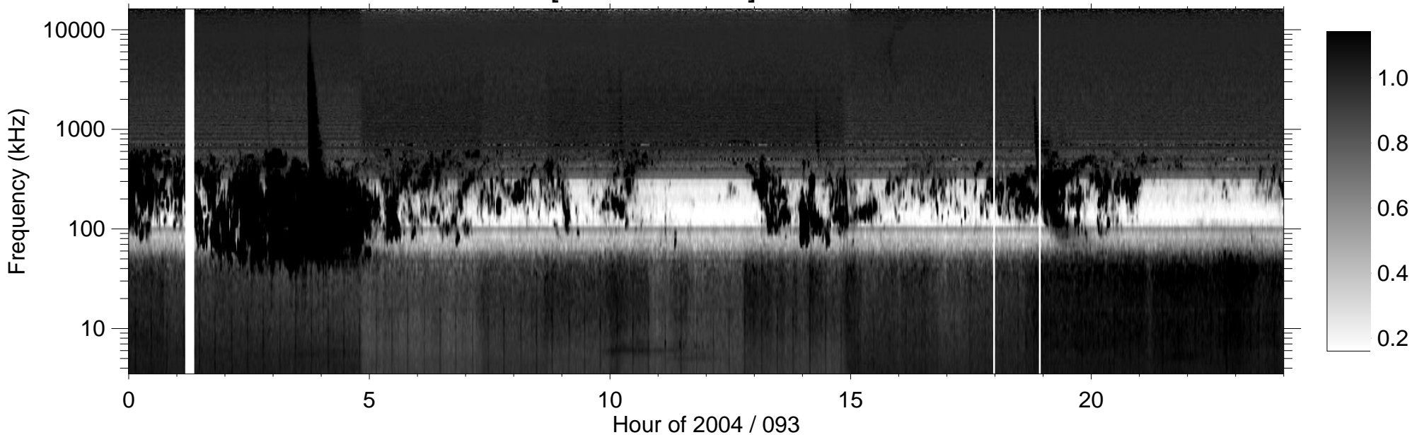
RPWS [ABCH1H2/Ex] (-B) 2004/04/02
