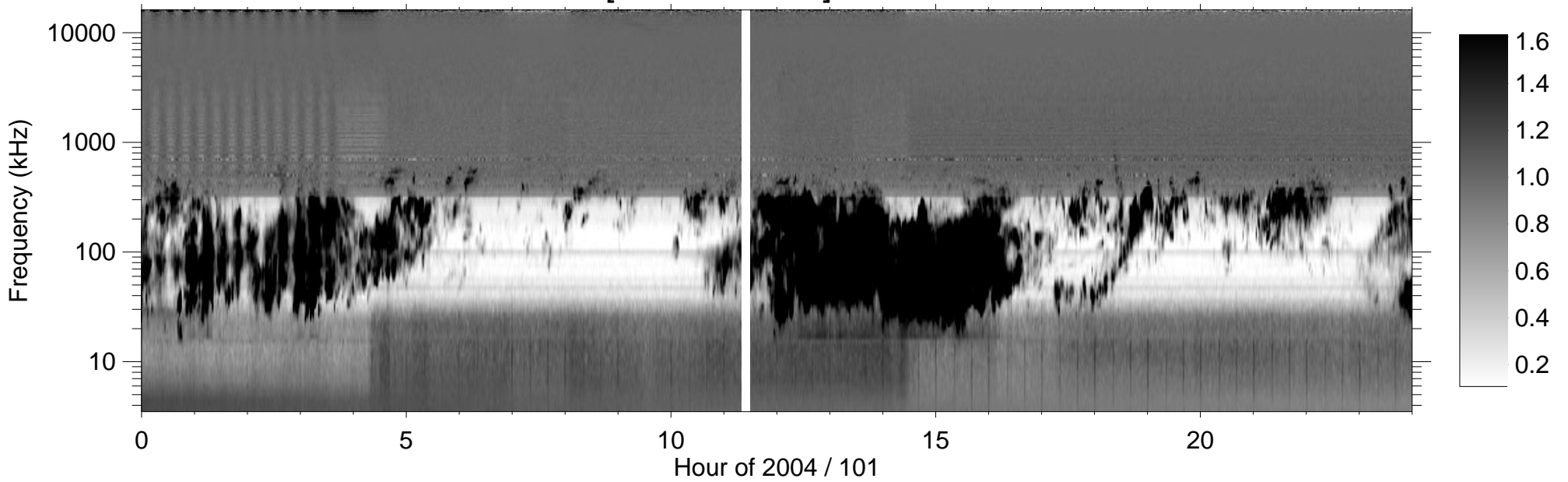
RPWS [ABCH1H2/Ex] (-B) 2004/04/10
