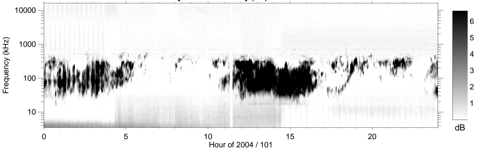
RPWS [ABCH1H2/Ex] (-B) 2004/04/10
