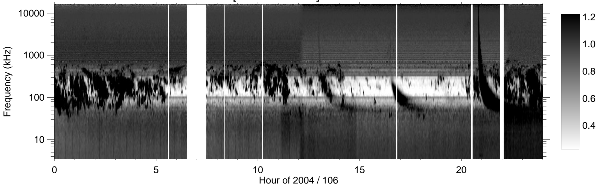
RPWS [ABCH1H2/Ex] (-B) 2004/04/15
