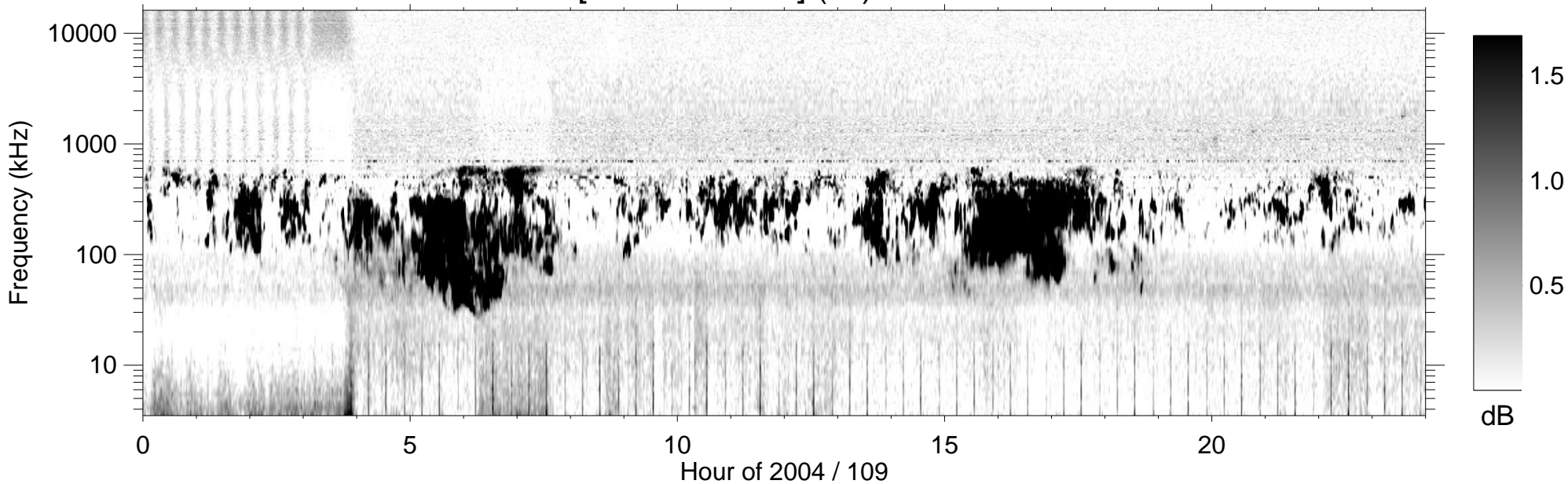
RPWS [ABCH1H2/Ex] (-B) 2004/04/18
