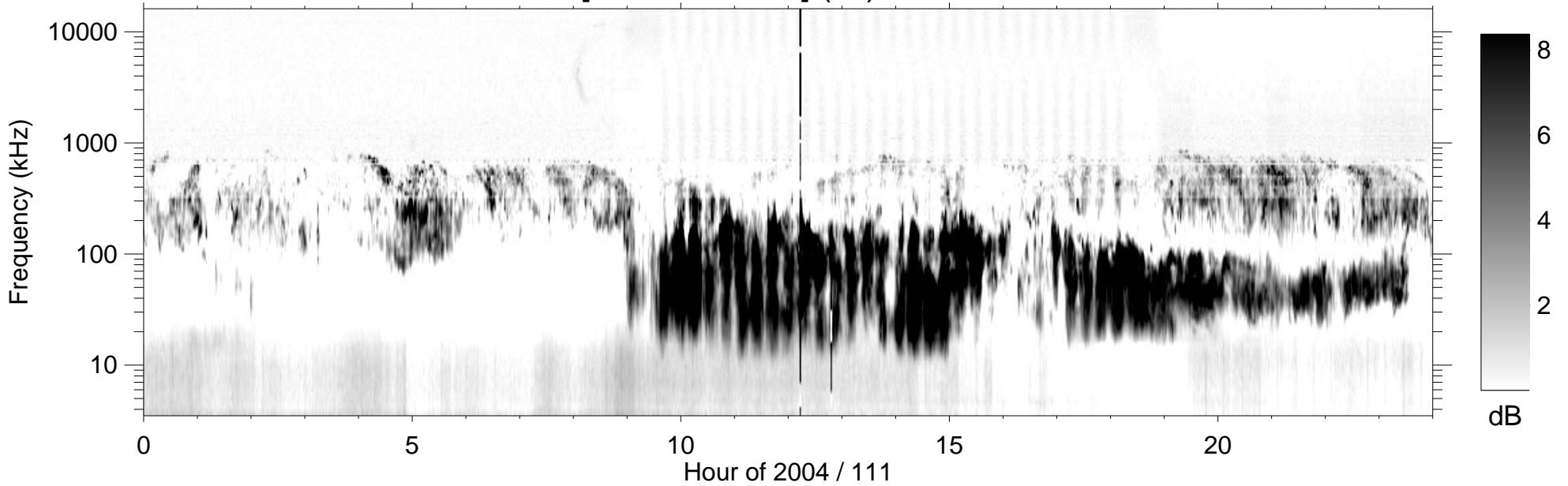
RPWS [ABCH1H2/Ex] (-B) 2004/04/20
