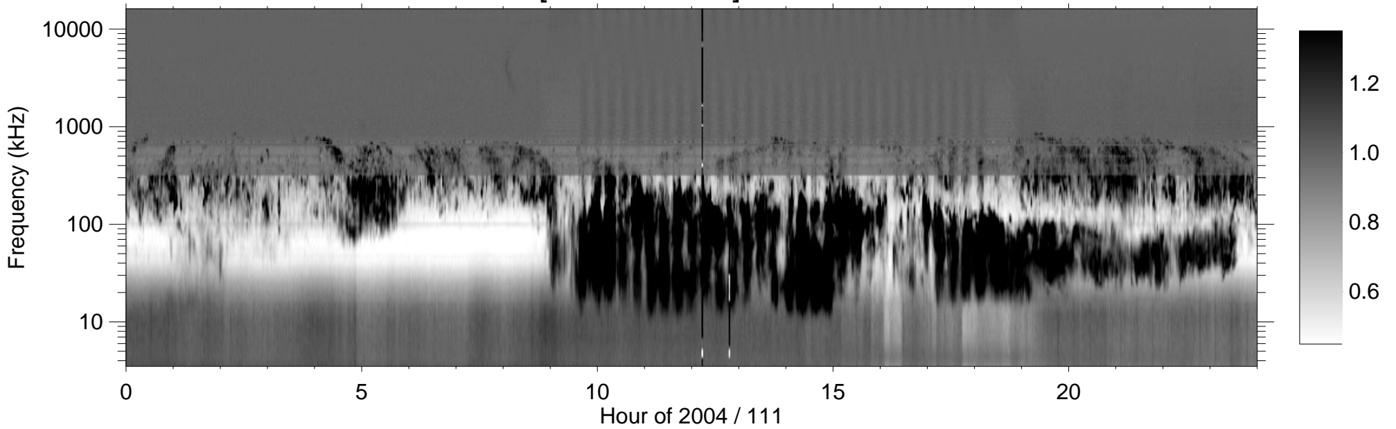
RPWS [ABCH1H2/Ex] (-B) 2004/04/20
