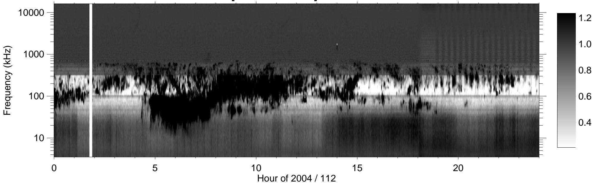
RPWS [ABCH1H2/Ex] (-B) 2004/04/21
