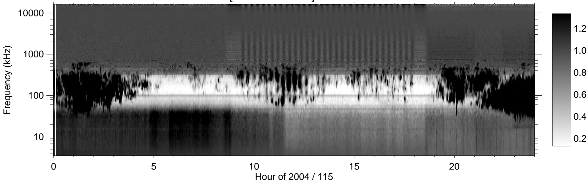
RPWS [ABCH1H2/Ex] (-B) 2004/04/24
