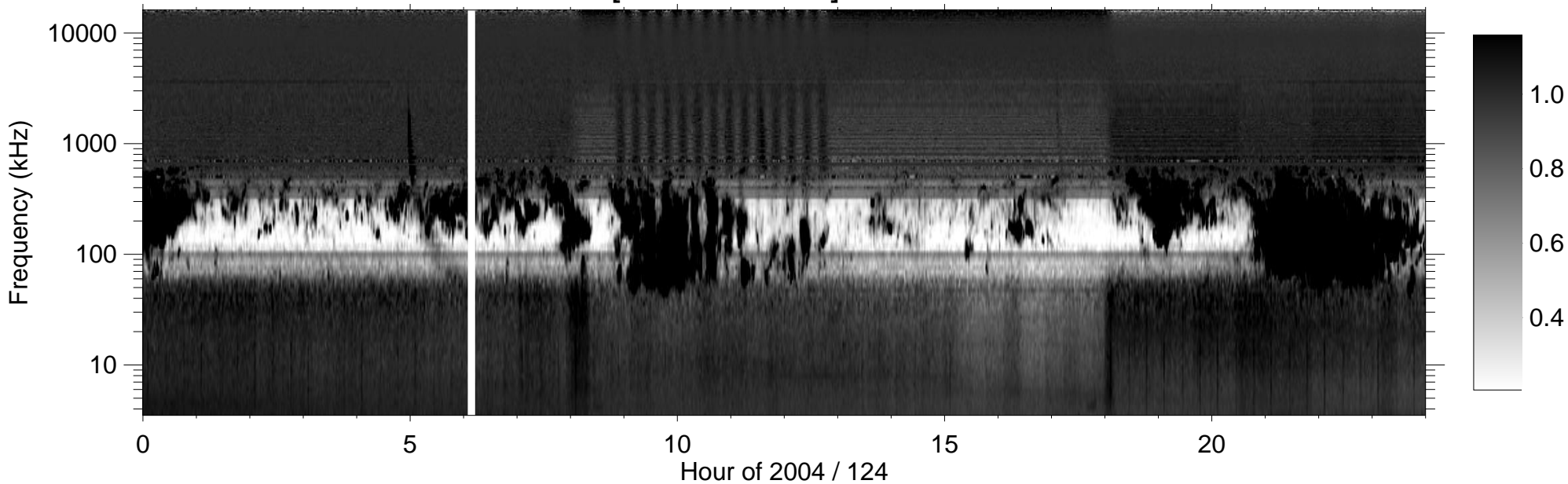
RPWS [ABCH1H2/Ex] (-B) 2004/05/03
