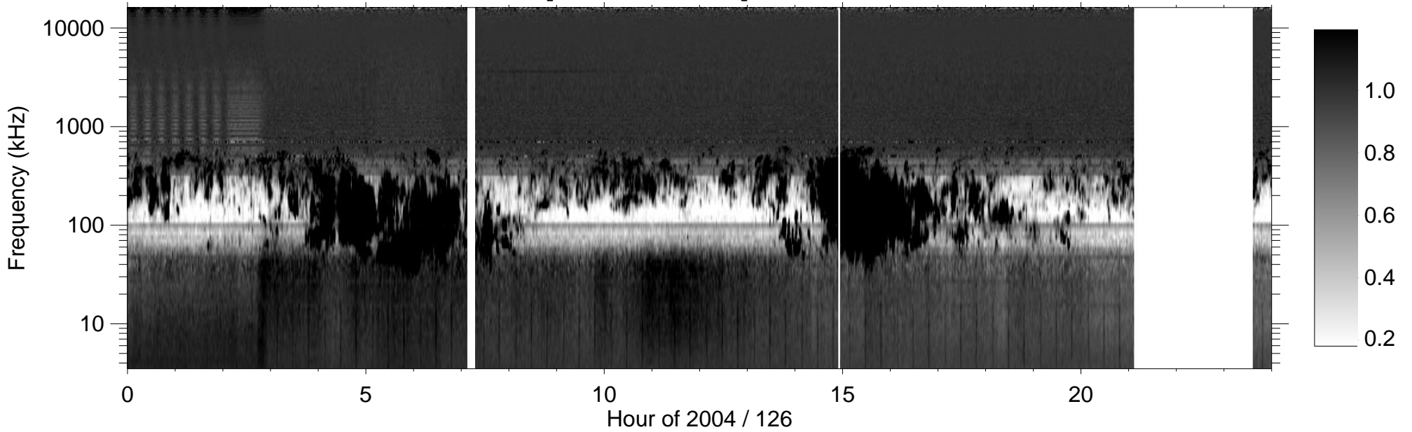
RPWS [ABCH1H2/Ex] (-B) 2004/05/05
