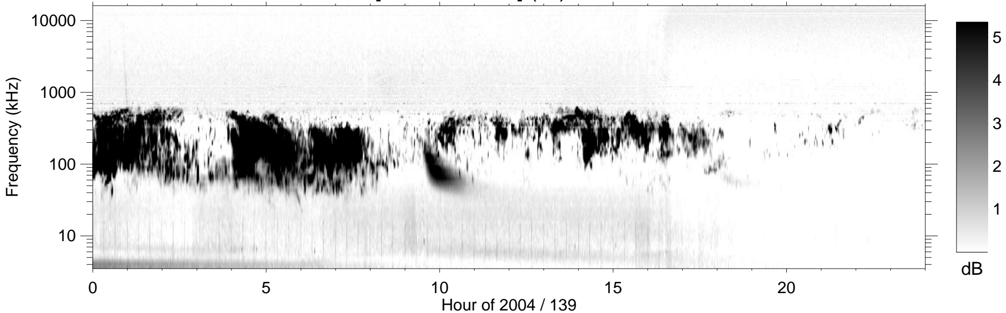
RPWS [ABCH1H2/Ex] (-B) 2004/05/18
