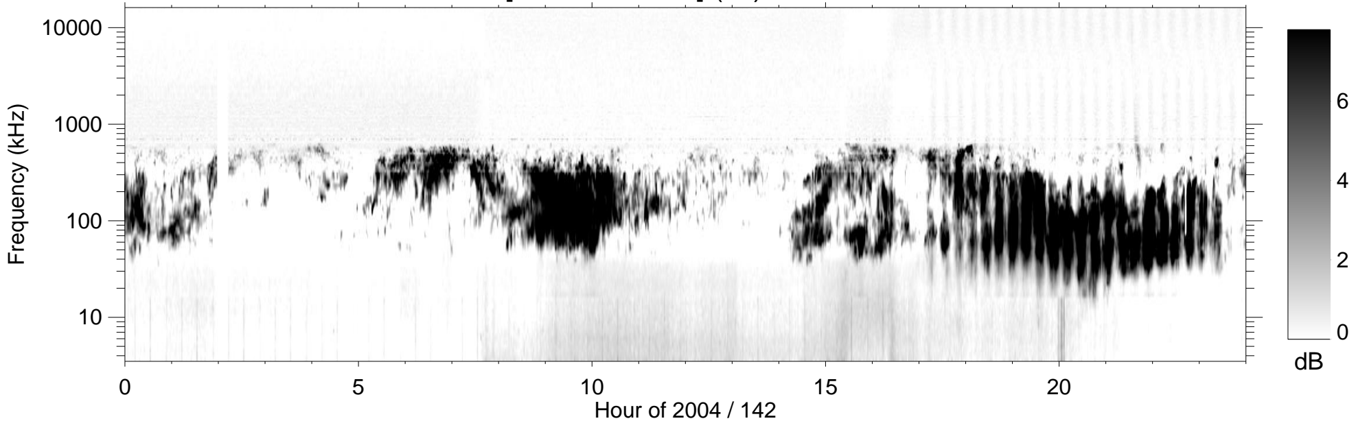
RPWS [ABCH1H2/Ex] (-B) 2004/05/21
