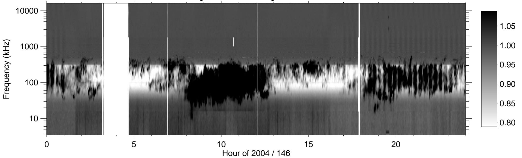
RPWS [ABCH1H2/Ex] (-B) 2004/05/25
