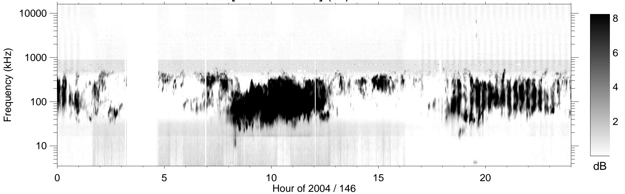
RPWS [ABCH1H2/Ex] (-B) 2004/05/25
