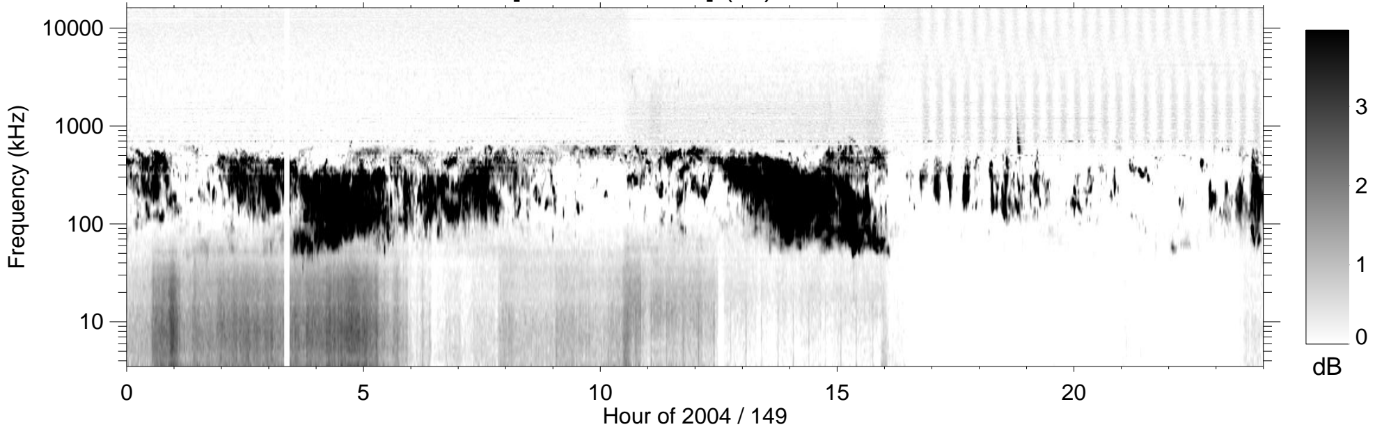
RPWS [ABCH1H2/Ex] (-B) 2004/05/28
