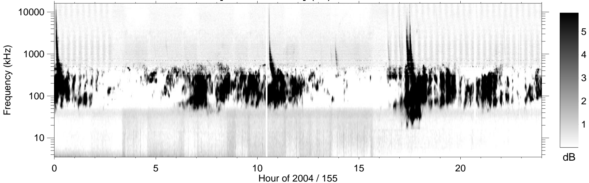
RPWS [ABCH1H2/Ex] (-B) 2004/06/03
