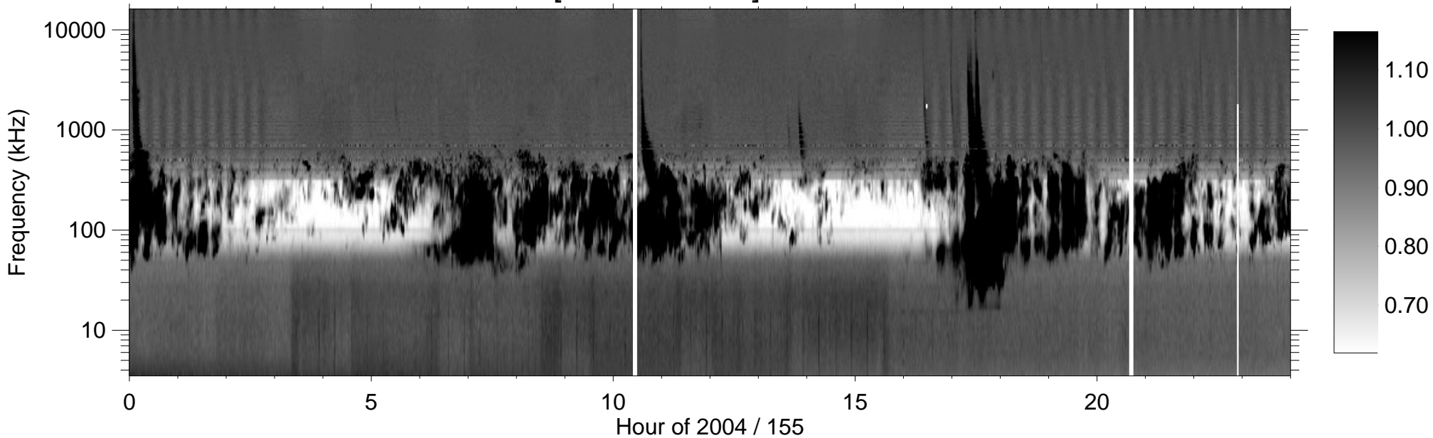
RPWS [ABCH1H2/Ex] (-B) 2004/06/03
