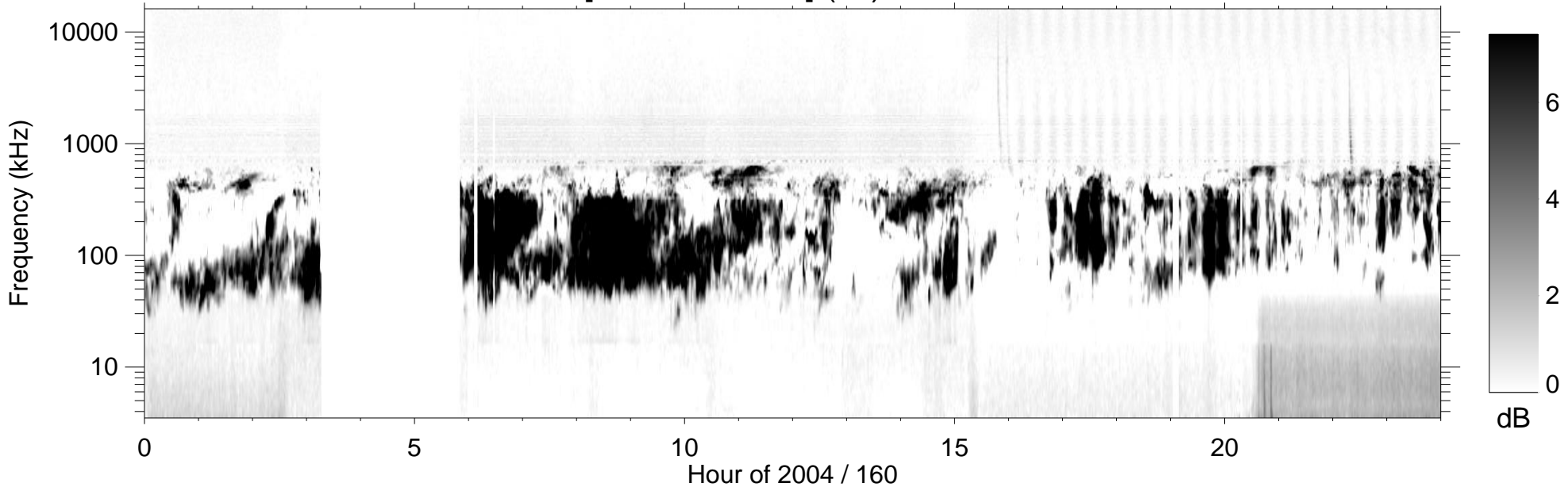
RPWS [ABCH1H2/Ex] (-B) 2004/06/08
