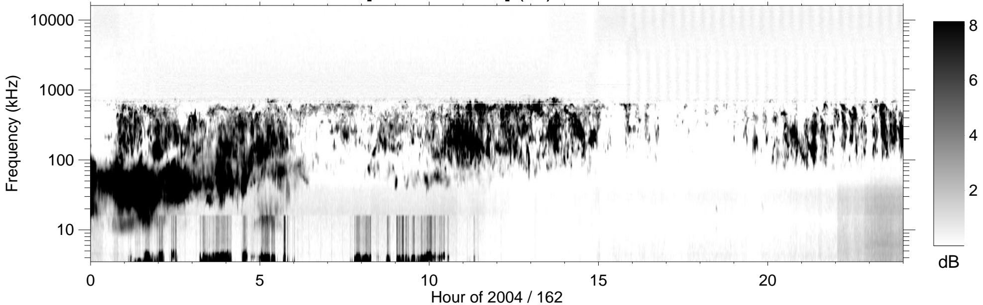
RPWS [ABCH1H2/Ex] (-B) 2004/06/10
