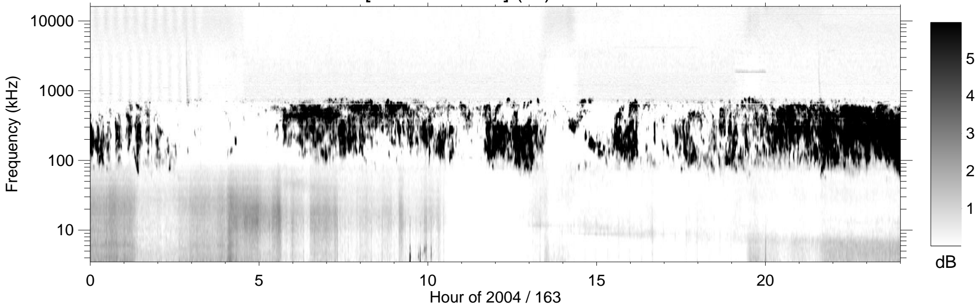
RPWS [ABCH1H2/Ex] (-B) 2004/06/11
