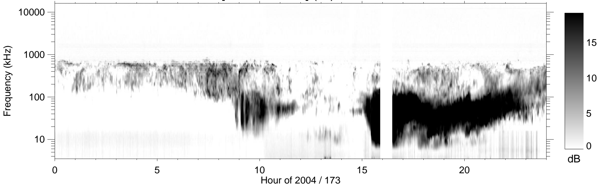
RPWS [ABCH1H2/Ex] (-B) 2004/06/21
