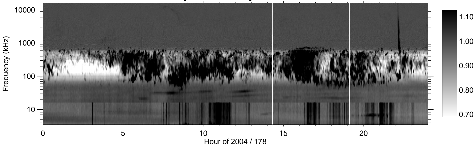
RPWS [ABCH1H2/Ex] (-B) 2004/06/26
