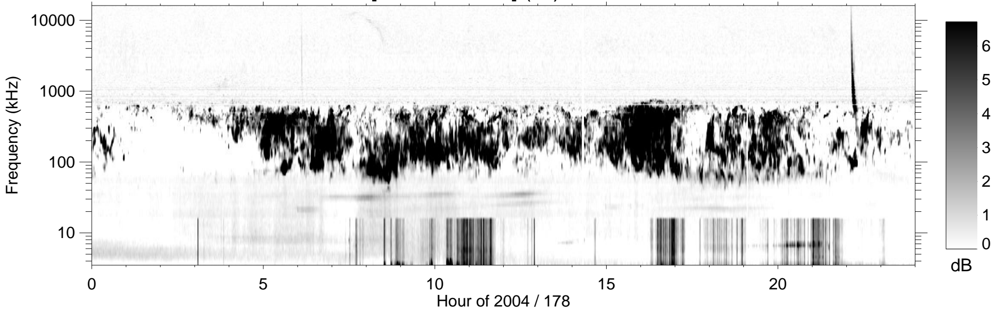
RPWS [ABCH1H2/Ex] (-B) 2004/06/26
