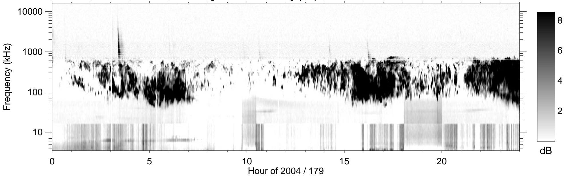
RPWS [ABCH1H2/Ex] (-B) 2004/06/27
