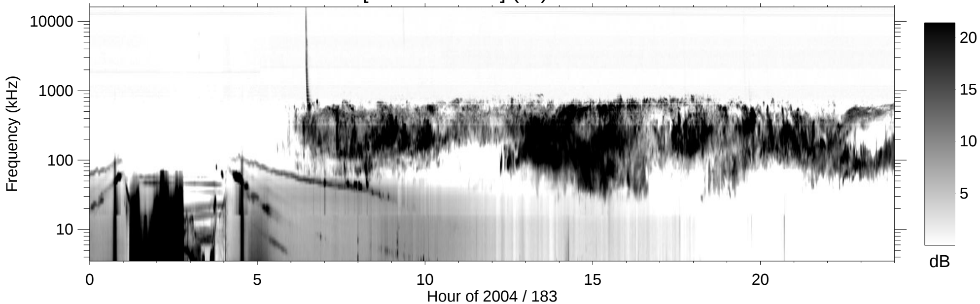
RPWS [ABCH1H2/Ex] (-B) 2004/07/01
