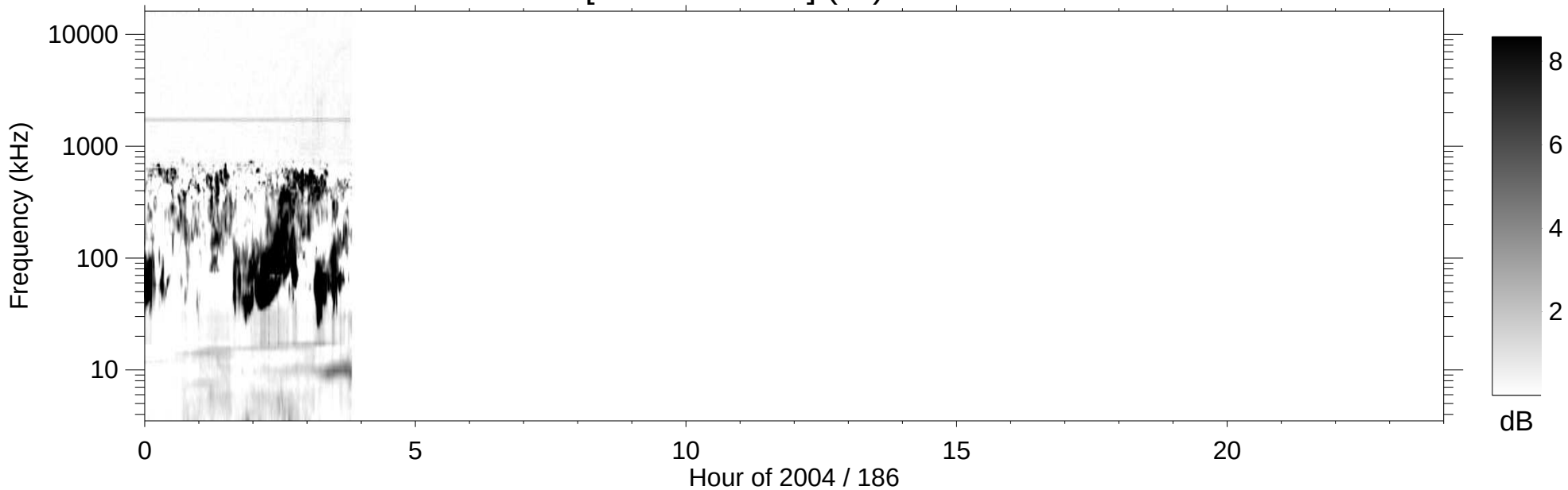
RPWS [ABCH1H2/Ex] (-B) 2004/07/04
