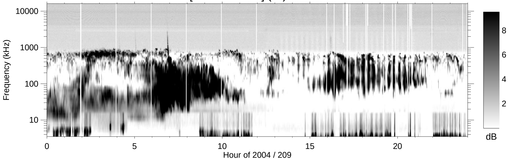
RPWS [ABCH1H2/Ex] (-B) 2004/07/27
