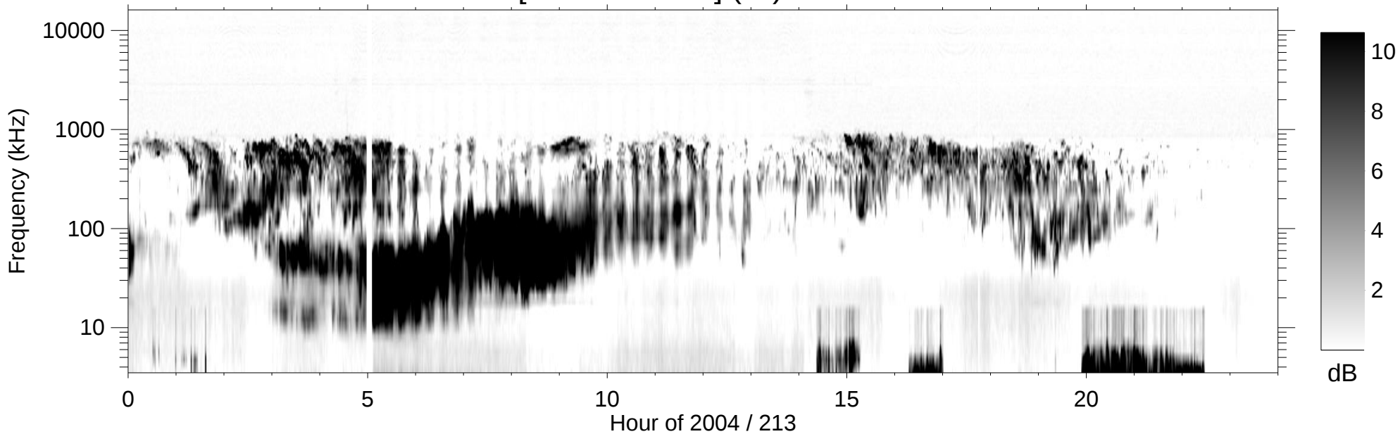
RPWS [ABCH1H2/Ex] (-B) 2004/07/31
