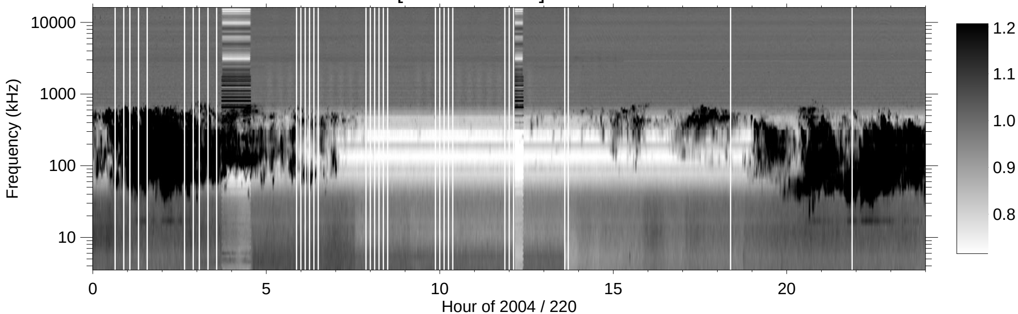
RPWS [ABCH1H2/Ex] (-B) 2004/08/07
