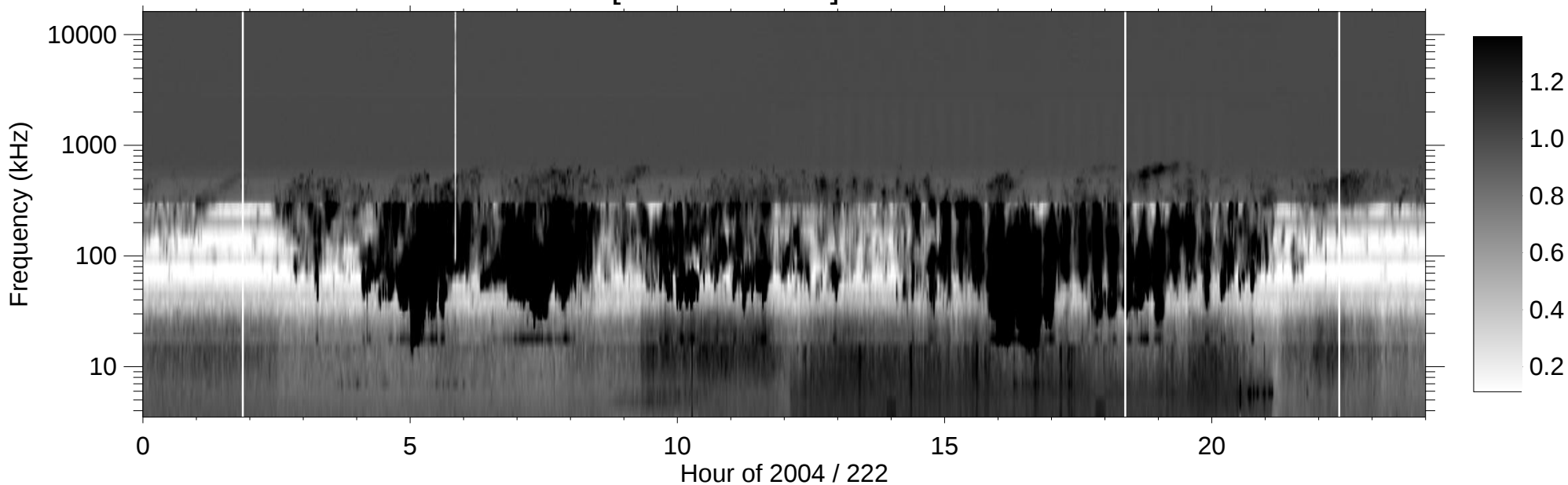
RPWS [ABCH1H2/Ex] (-B) 2004/08/09
