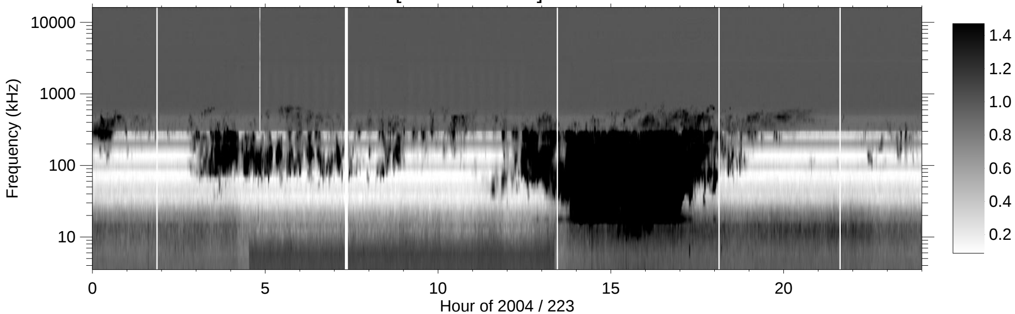
RPWS [ABCH1H2/Ex] (-B) 2004/08/10
