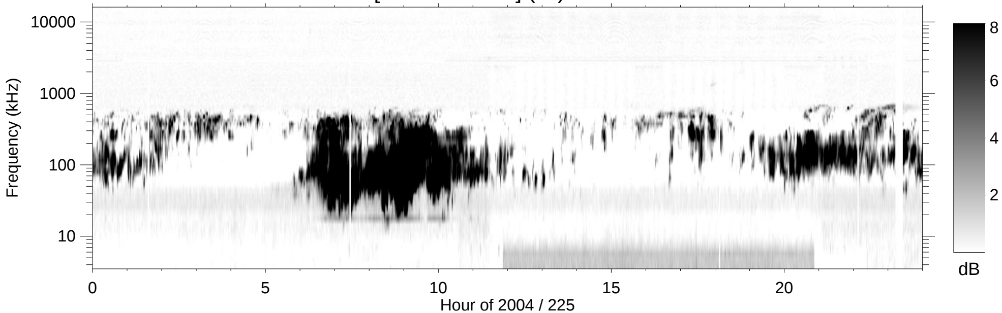
RPWS [ABCH1H2/Ex] (-B) 2004/08/12
