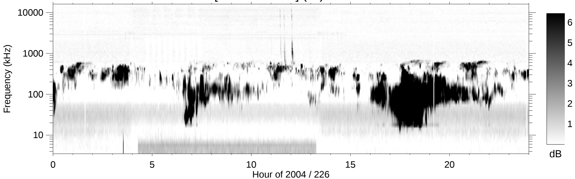
RPWS [ABCH1H2/Ex] (-B) 2004/08/13
