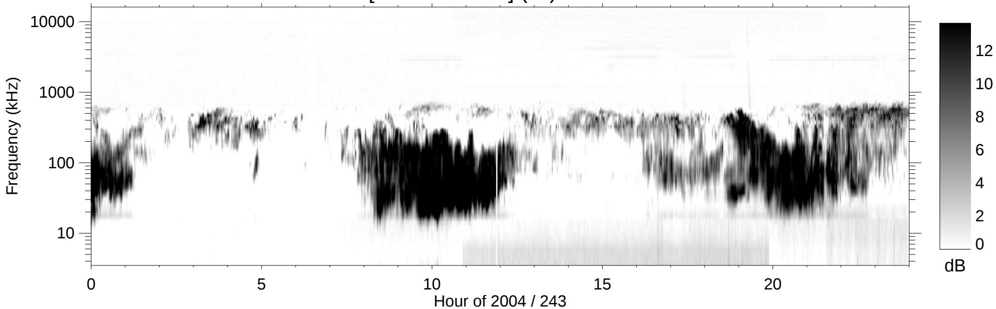
RPWS [ABCH1H2/Ex] (-B) 2004/08/30
