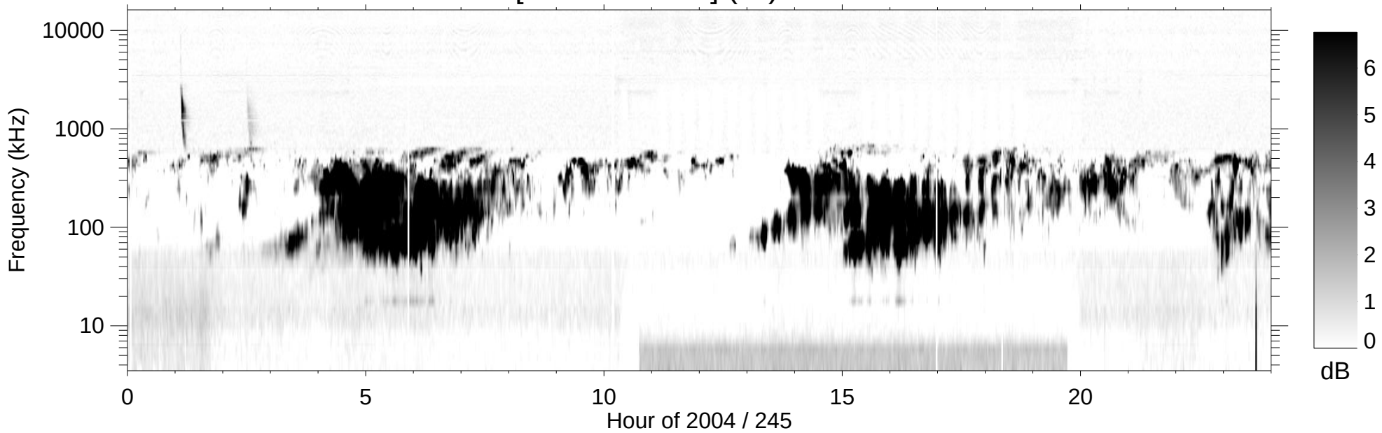
RPWS [ABCH1H2/Ex] (-B) 2004/09/01
