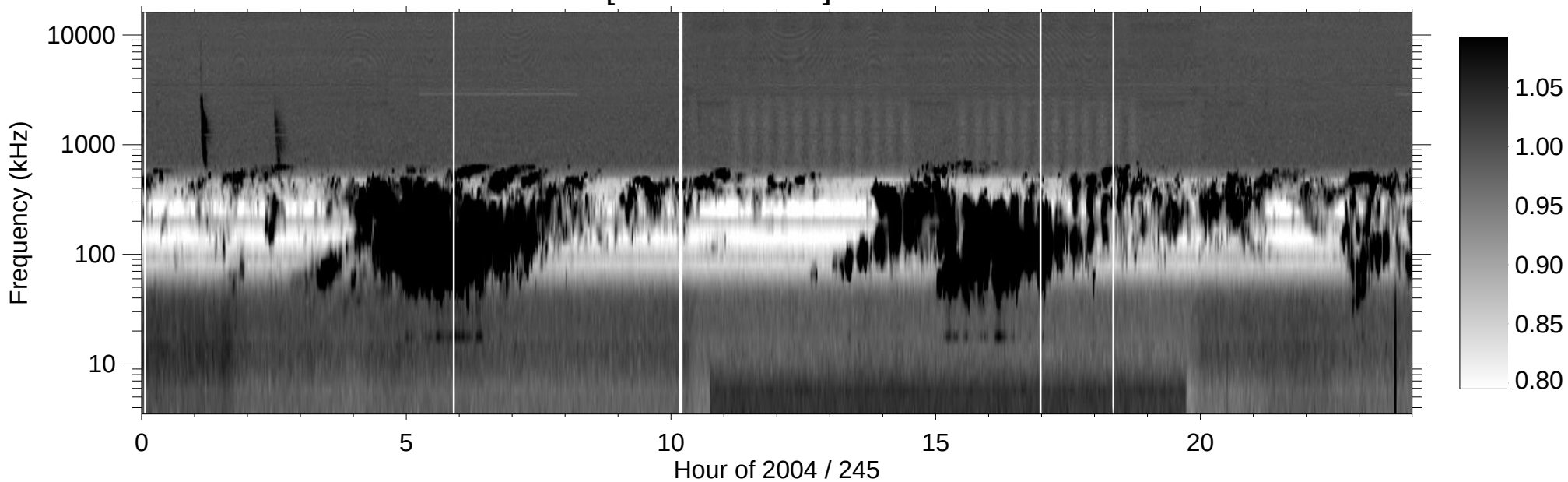
RPWS [ABCH1H2/Ex] (-B) 2004/09/01
