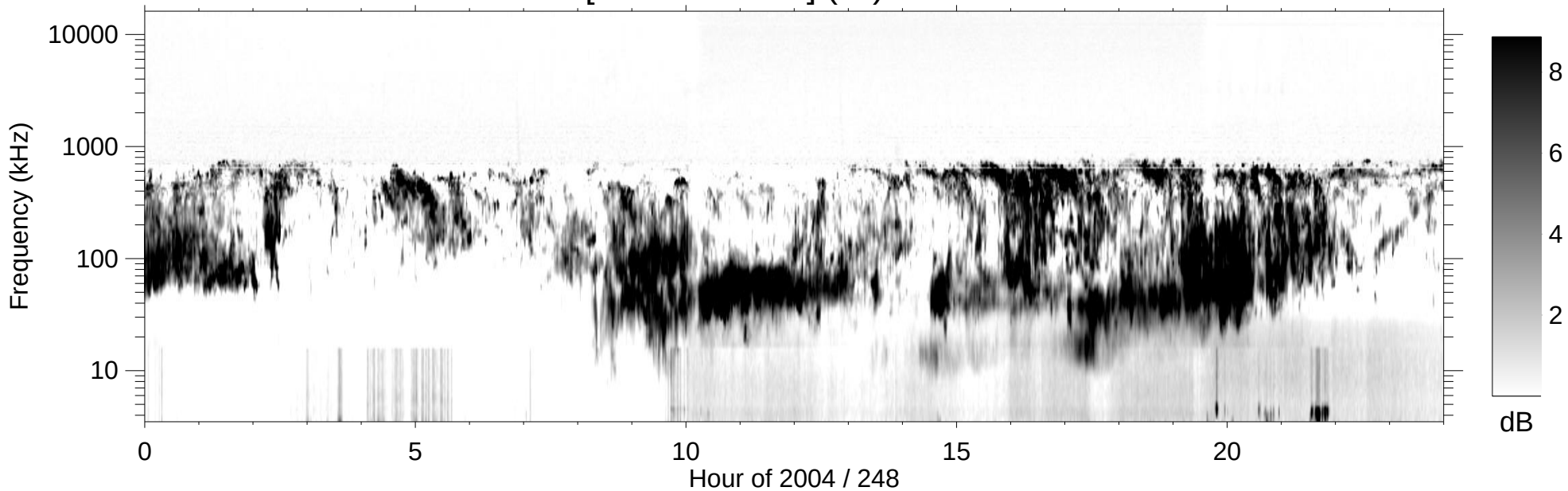
RPWS [ABCH1H2/Ex] (-B) 2004/09/04
