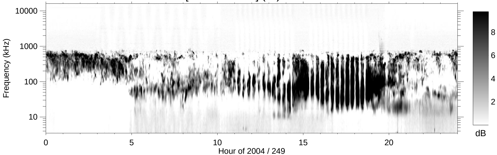
RPWS [ABCH1H2/Ex] (-B) 2004/09/05
