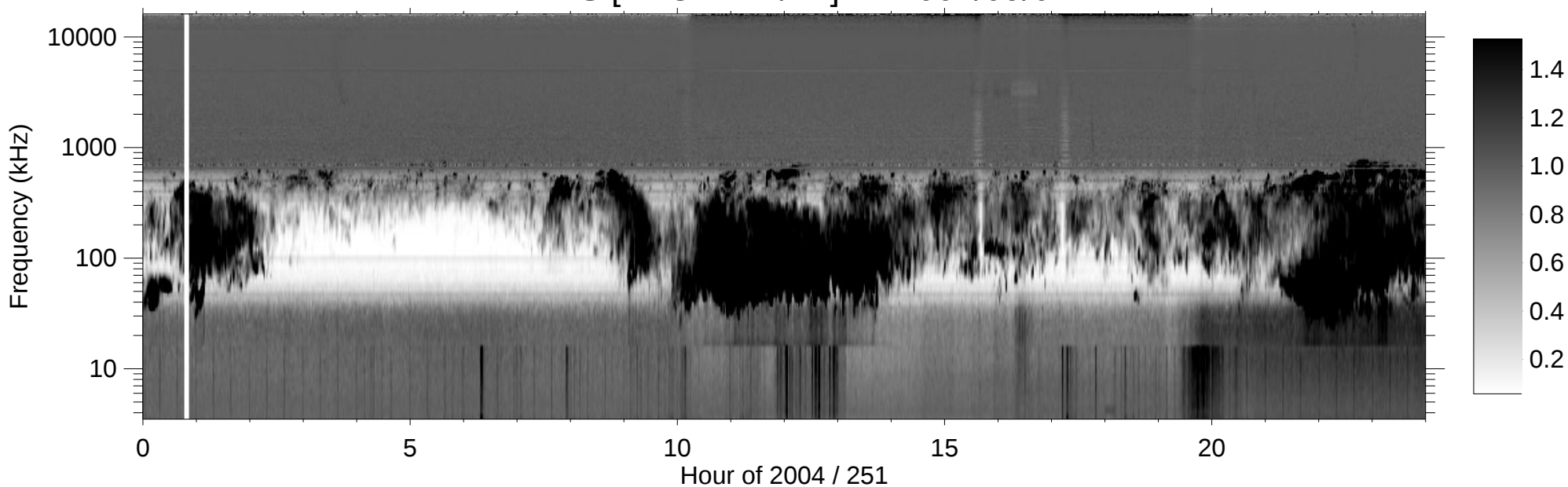
RPWS [ABCH1H2/Ex] (-B) 2004/09/07
