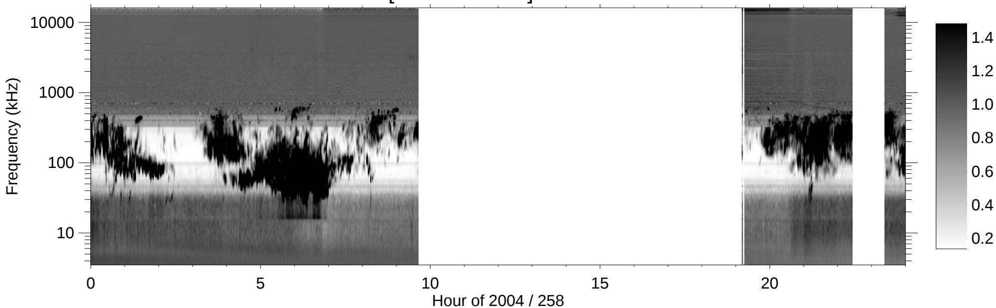
RPWS [ABCH1H2/Ex] (-B) 2004/09/14
