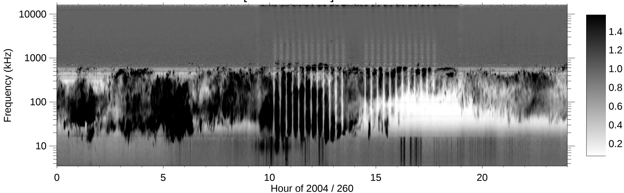
RPWS [ABCH1H2/Ex] (-B) 2004/09/16
