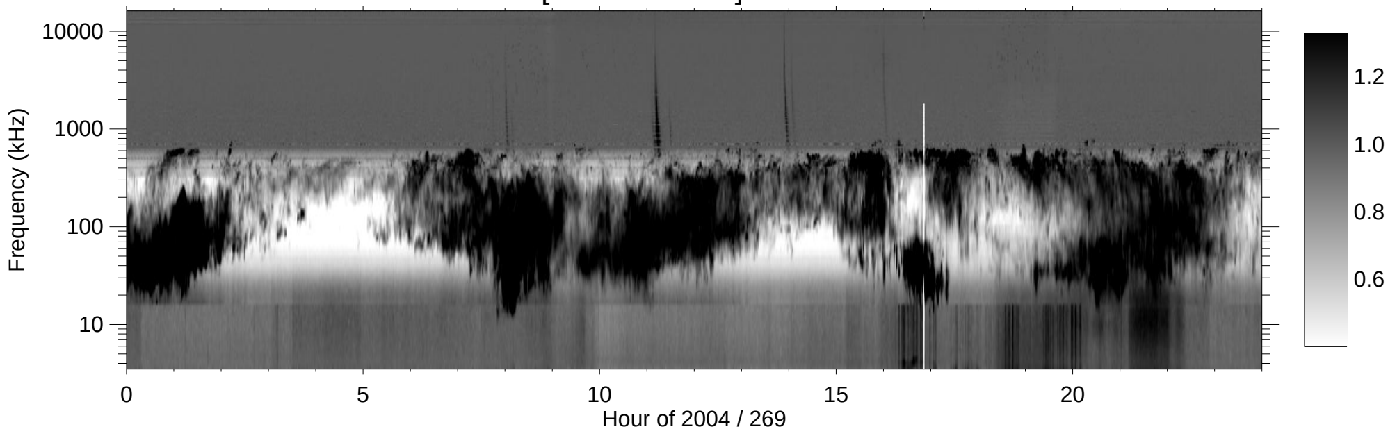
RPWS [ABCH1H2/Ex] (-B) 2004/09/25
