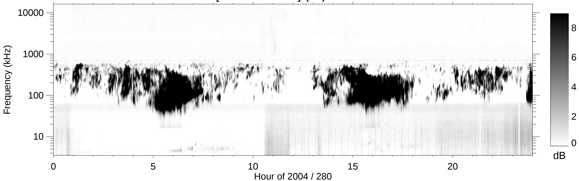
RPWS [ABCH1H2/Ex] (-B) 2004/10/06
