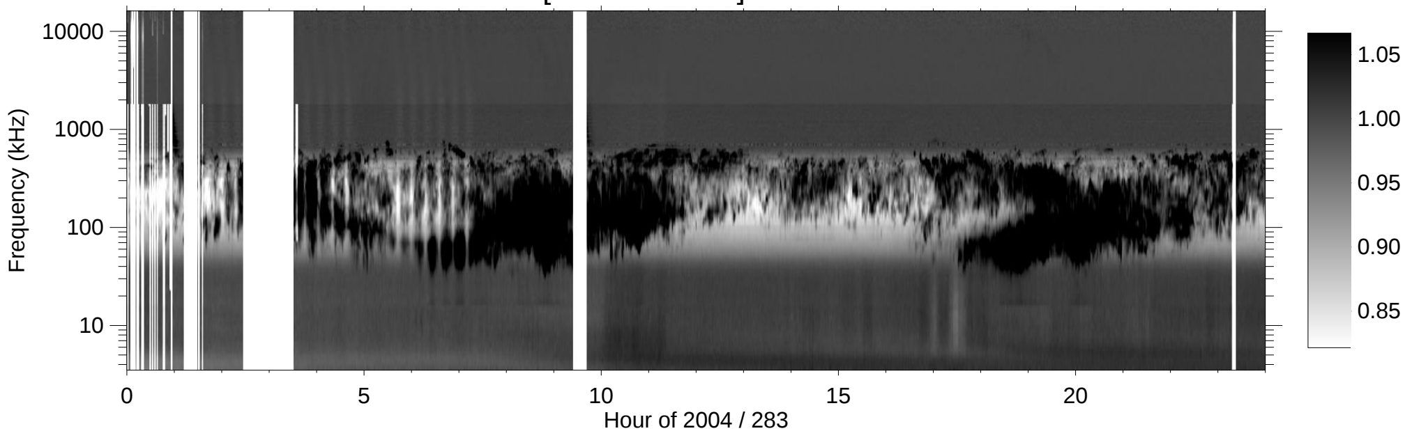
RPWS [ABCH1H2/Ex] (-B) 2004/10/09
