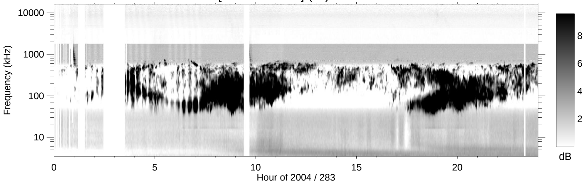
RPWS [ABCH1H2/Ex] (-B) 2004/10/09
