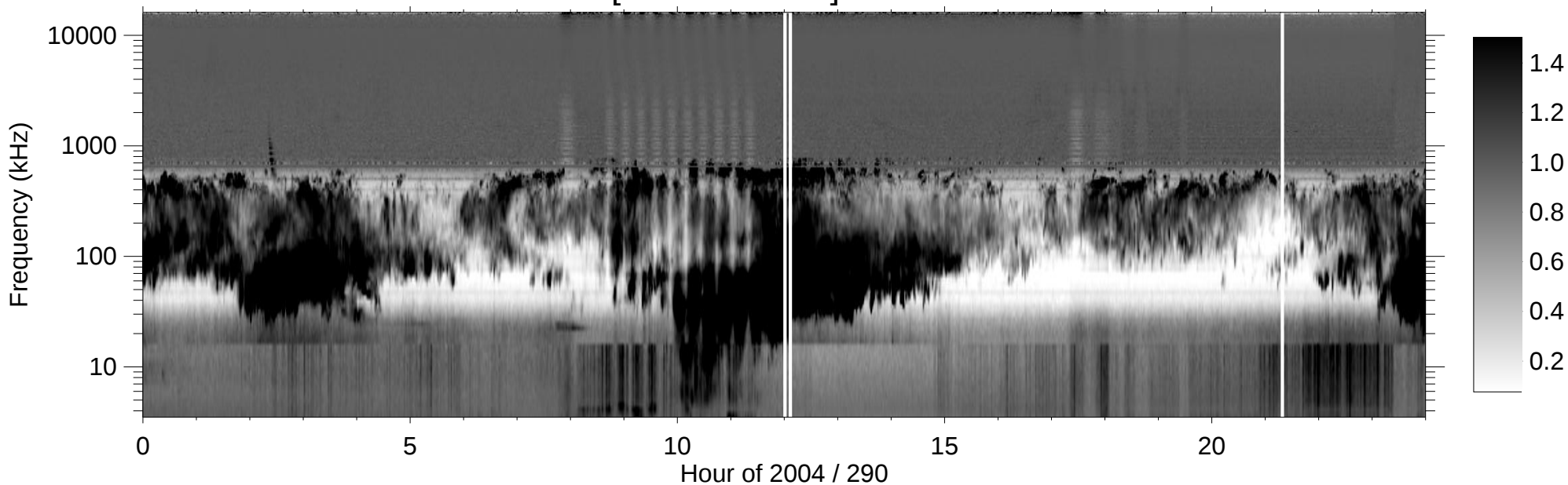
RPWS [ABCH1H2/Ex] (-B) 2004/10/16
