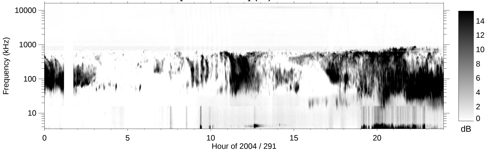
RPWS [ABCH1H2/Ex] (-B) 2004/10/17
