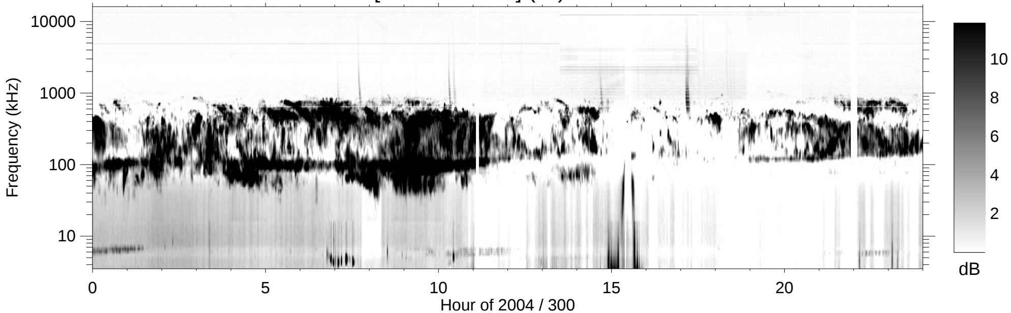
RPWS [ABCH1H2/Ex] (-B) 2004/10/26
