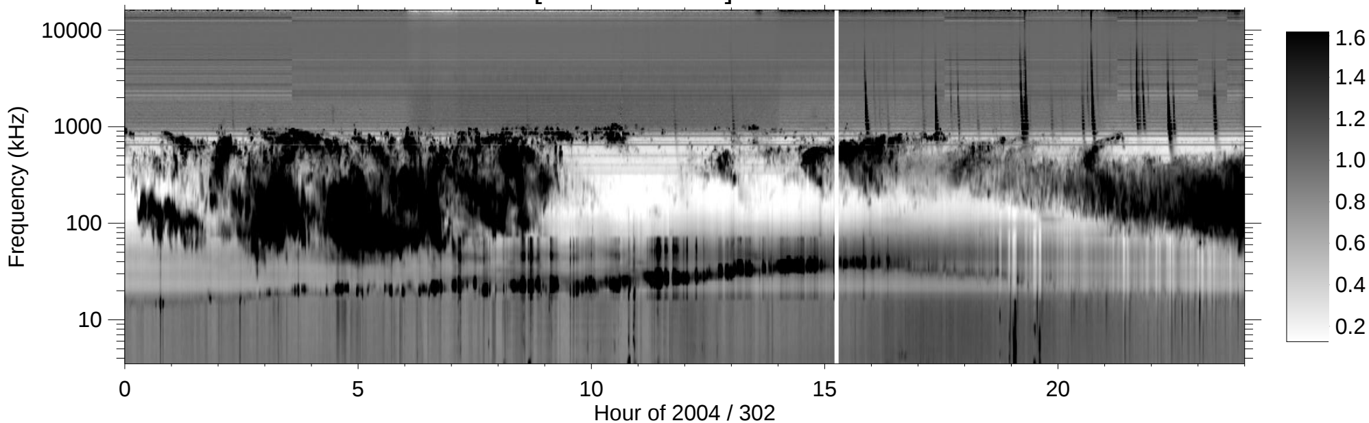
RPWS [ABCH1H2/Ex] (-B) 2004/10/28
