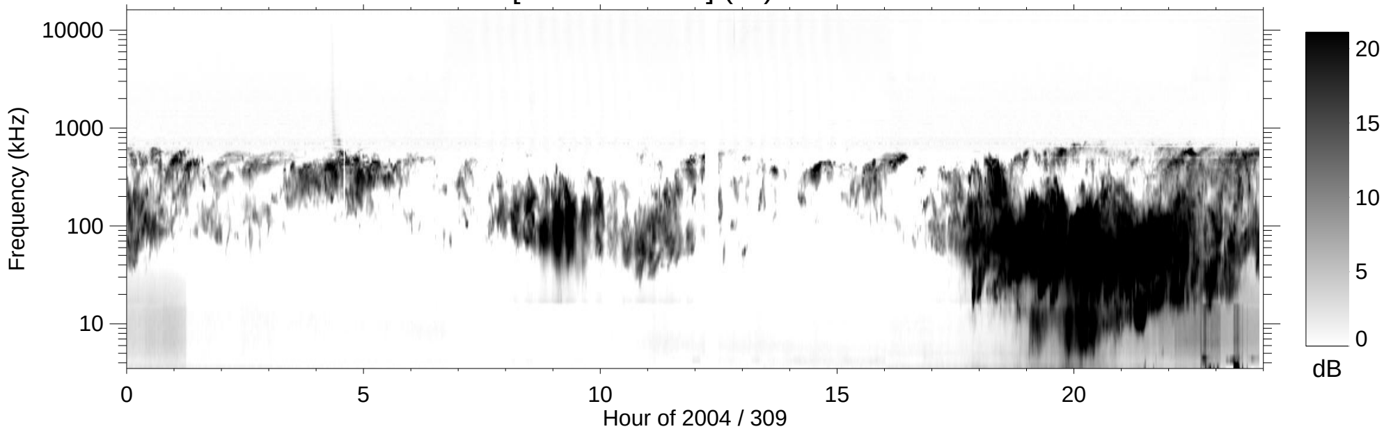
RPWS [ABCH1H2/Ex] (-B) 2004/11/04
