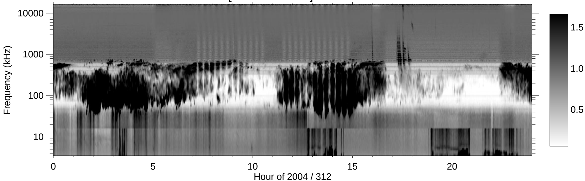
RPWS [ABCH1H2/Ex] (-B) 2004/11/07
