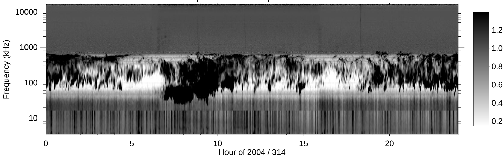
RPWS [ABCH1H2/Ex] (-B) 2004/11/09
