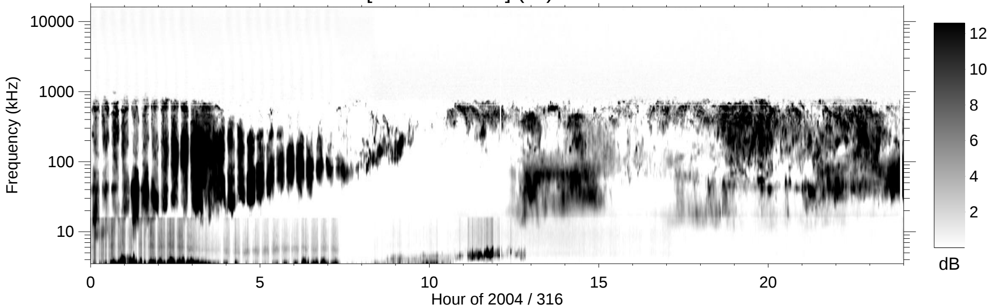
RPWS [ABCH1H2/Ex] (-B) 2004/11/11
