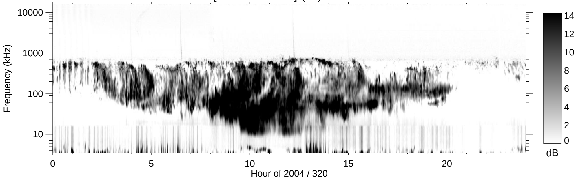
RPWS [ABCH1H2/Ex] (-B) 2004/11/15
