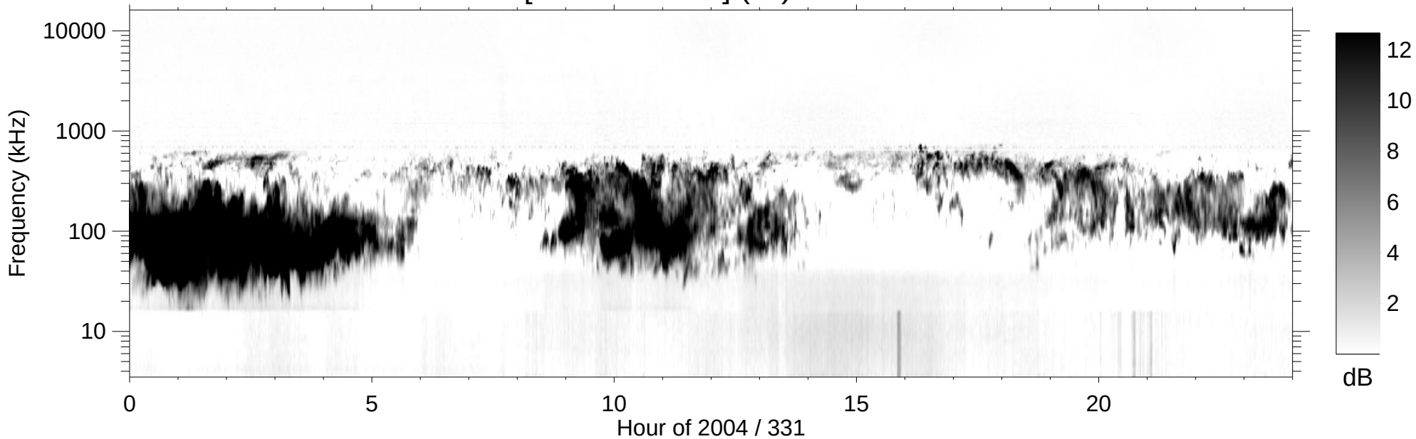
RPWS [ABCH1H2/Ex] (-B) 2004/11/26
